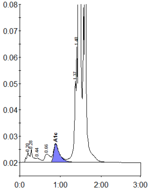
Peak table - ID: 10410009
